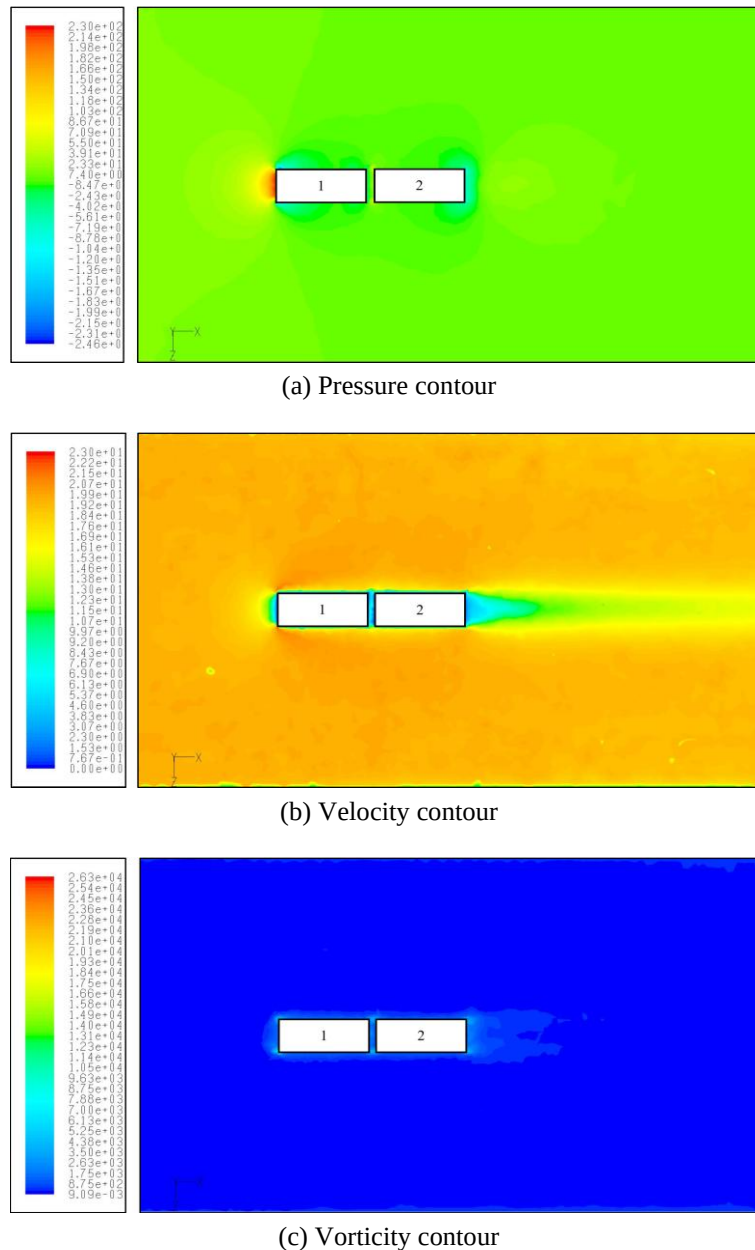
Fig. 9 The CFD simulation results at a flow rate of U = 20 \text{ m/s} ( Re = 54726 ), with L/D = 0.227 arranged in tandem
