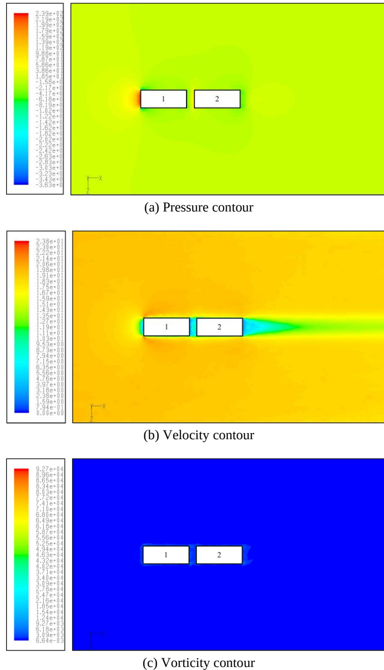
Fig. 10 The CFD simulation results at a flow rate of U = 20 m/s ( Re = 54726 ), with L/D = 0.455 arranged in tandem
