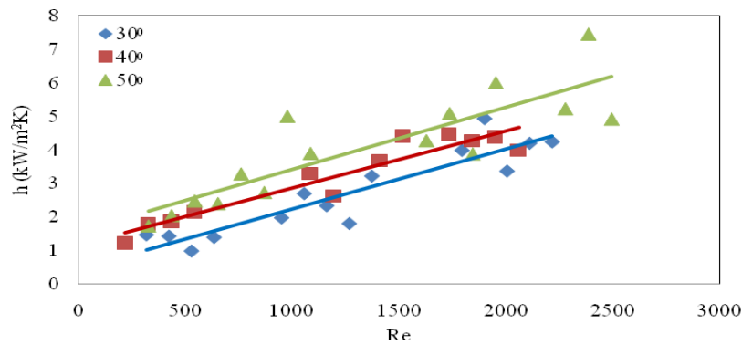
Fig. 14 Heat transfer coefficient Vs Reynolds number for 30 0 , 40 0 and 50 0 corrugation angles with water as test fluid
