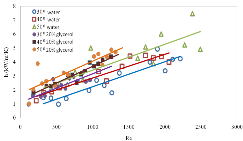
Fig. 16 Heat transfer coefficient Vs Reynolds number for 30 0 , 40 0 and 50 0 corrugation angles with water and 20% glycerol solution as test fluids
