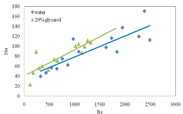
Fig. 13 Nusselt number Vs Reynolds number for 50° corrugation angle with water and 20% glycerol solution as test fluids
