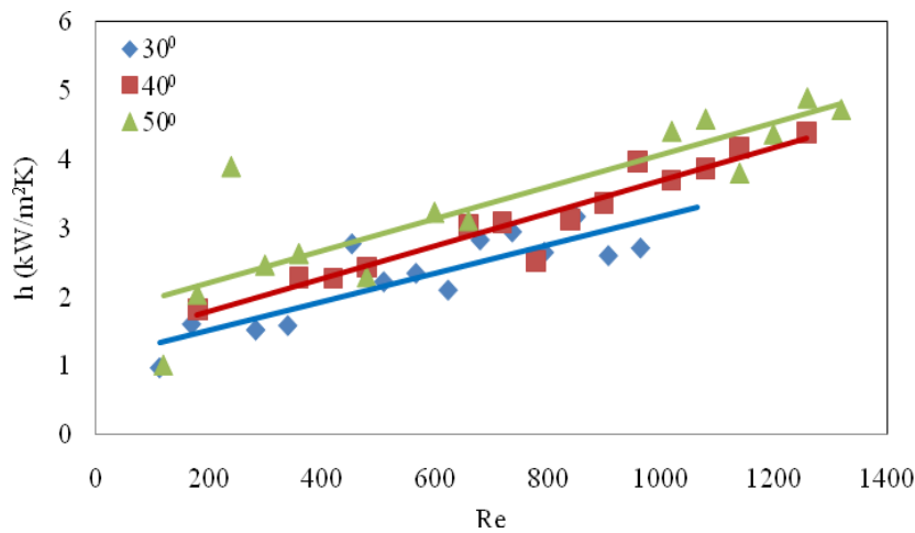
Fig. 15 Heat transfer coefficient Vs Reynolds number for 30 0 , 40 0 and 50 0 corrugation angles with 20% glycerol solution as test fluid
