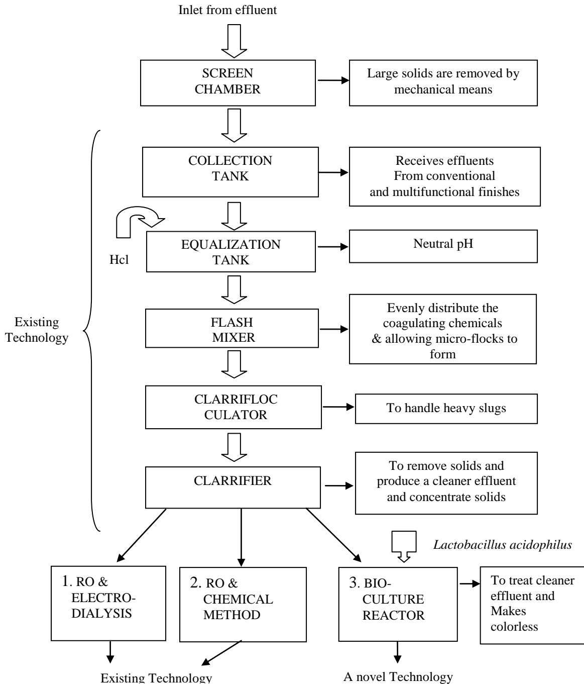
Fig. 1 Flow Chart for Effluent Treatment using Lactobacillus acidophilus bacterium
