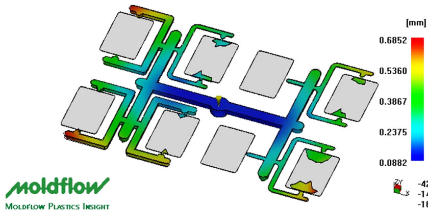
Fig. 11 Schematic of warpage phenomenon
