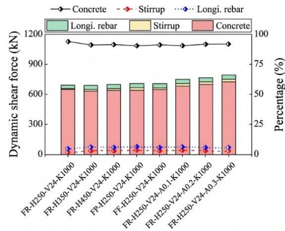
Fig. 9 Components of the shear force in RC columns at peak impact under a 1000 kN/mm impactor
