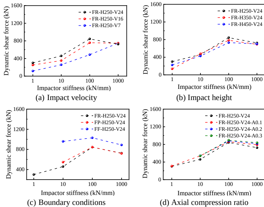
Fig. 8 Variation of the dynamic shear force with impactor stiffness for each simulation series
