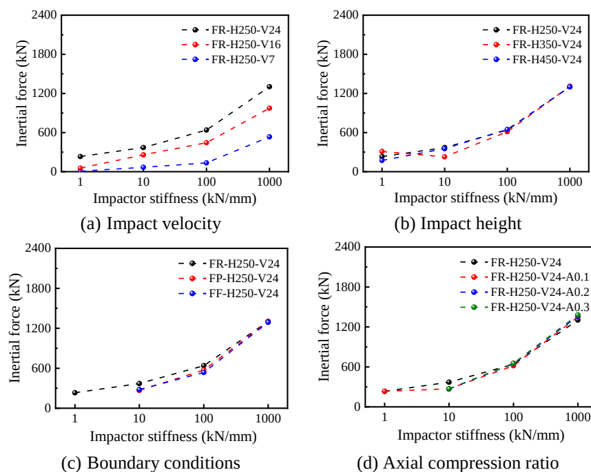
Fig. 10 Relationship between peak inertial force and impactor stiffness
