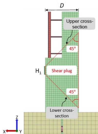
Fig. 4 Schematic diagram of shear plug within RC column
