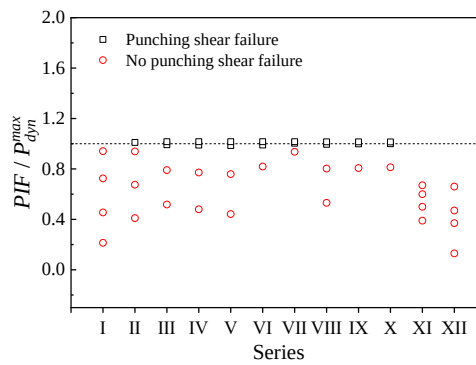
Fig. 11 Relationship between damage level of RC columns and the PIF/P_{dyn}^{max} ratio for every series
