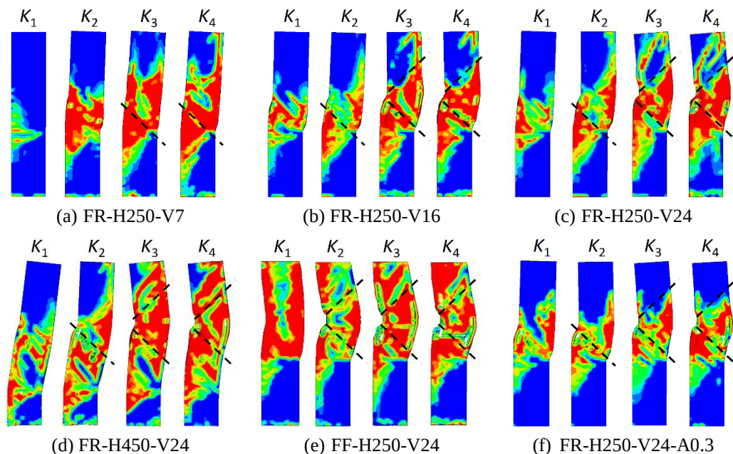
Fig. 5 Failure modes of six typical model series under representative impactor stiffnesses ( K_1 , K_2 , K_3 , and K_4 = 1, 10, 100 , and 1000 kN/mm, respectively)
