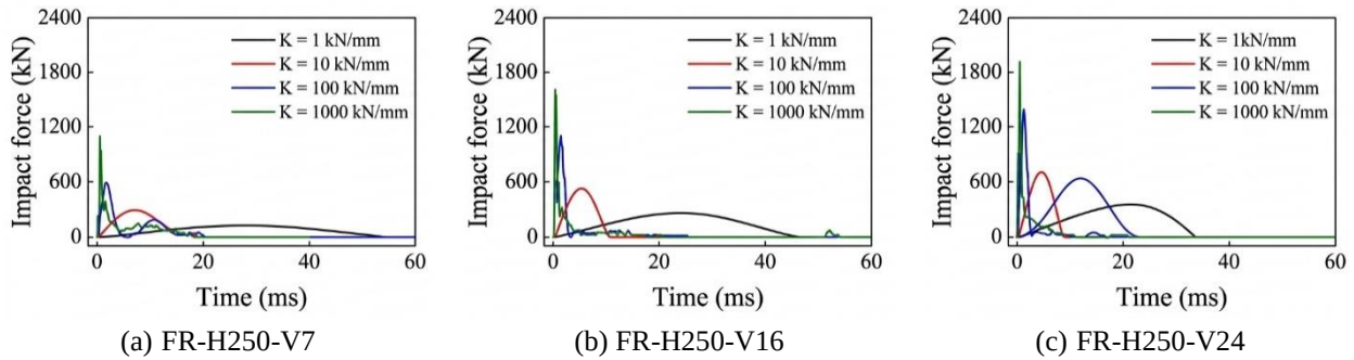
Fig. 6 Impact force time histories of FR-H250 series under different impactor stiffness
