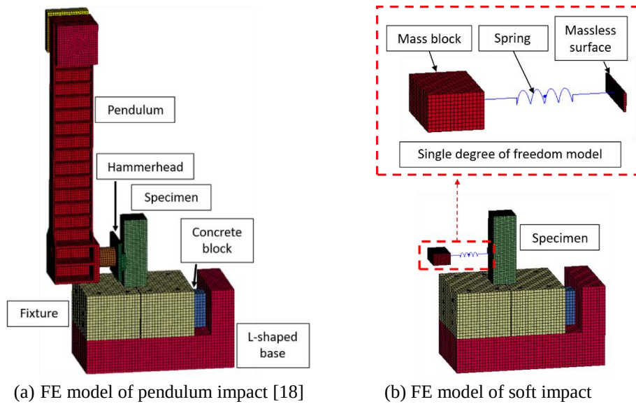
Fig. 1 Numerical analysis models of hard and soft impacts
