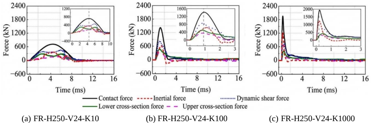
Fig. 7 Time histories of dynamic forces acting on FR-H250-V24 under different impactor stiffnesses
