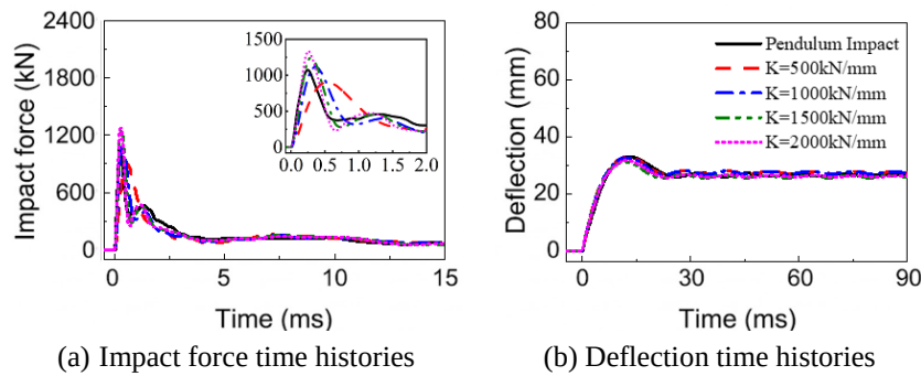
Fig. 2 Comparison of impact force and deflection time histories
