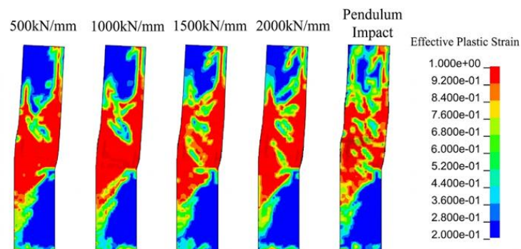
Fig. 3 Comparison of damage and failure modes of RC columns
