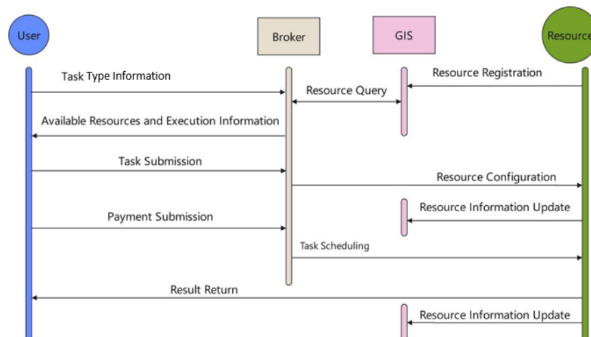
Fig. 7 Dynamic task resource configuration sequence
