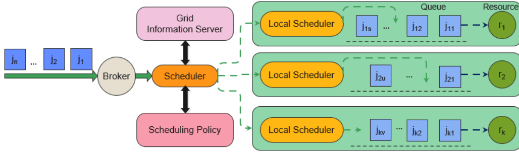
Fig. 1 Dynamic task scheduling model
