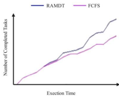
Fig. 9 Comparison between RAMDT and FCFS algorithms
