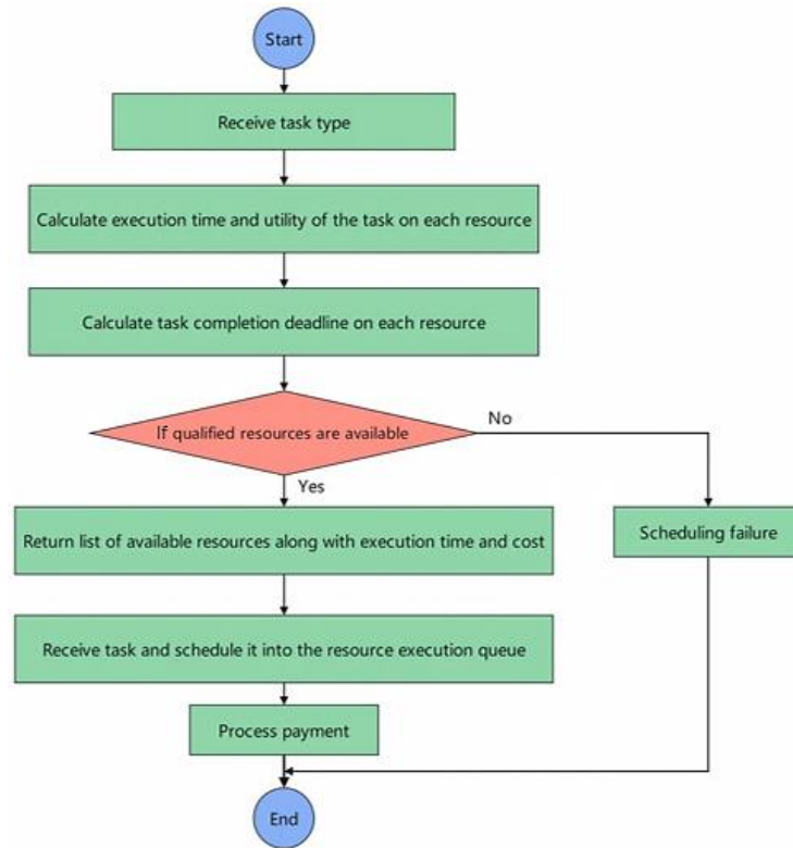
Fig. 6 The task scheduling process of the resource scheduling system
