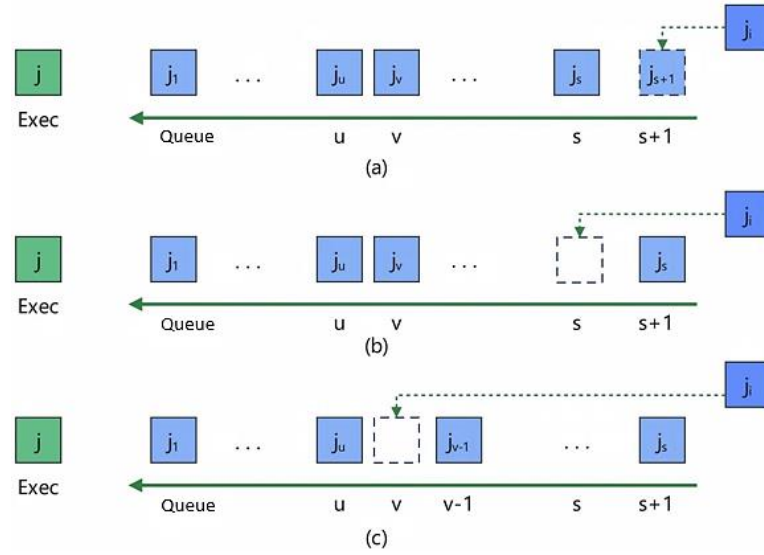
Fig. 2 User ranking in the queue based on submitted value
