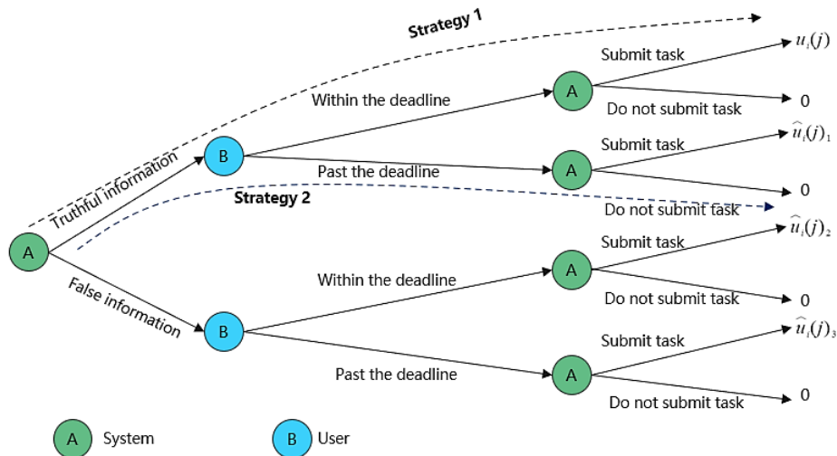
Fig. 4 Tree representation of user utility
