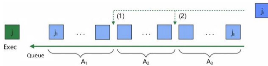
Fig. 3 Queue ordering based on the submitted task length
