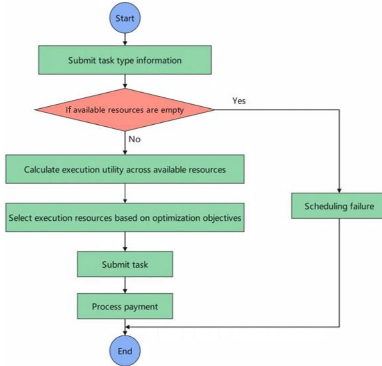
Fig. 5 User task strategy selection process
