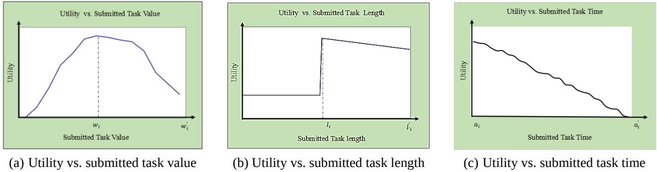
Fig. 8 Relationship between utility and submitted task value, length, and time
