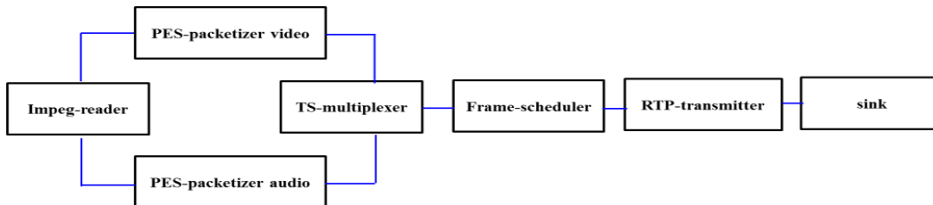
Fig. 10 SIRANNON network
