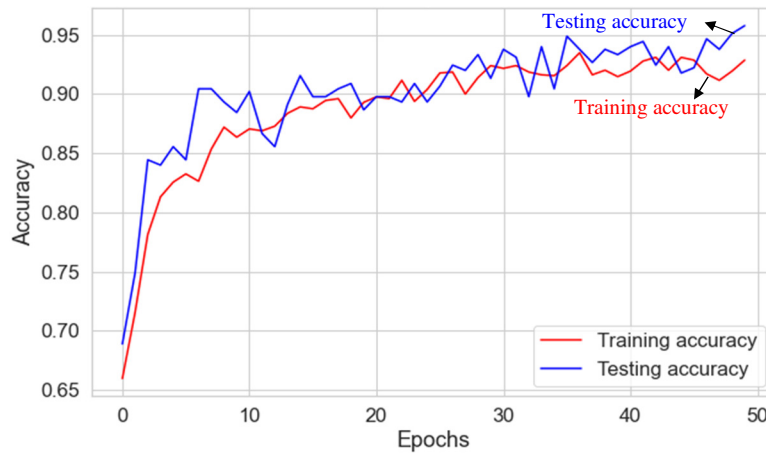
Fig. 2 Accuracy curves for the CNN
