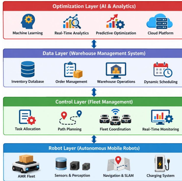
Fig. 2 Architecture of the proposed AMR-based smart warehouse system
