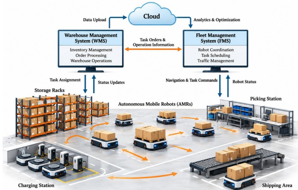
Fig. 1 Smart warehouse logistics system with AMRs
