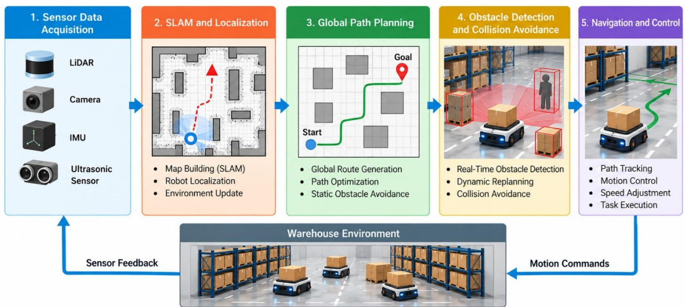
Fig. 3 Autonomous robot navigation and path planning workflow
